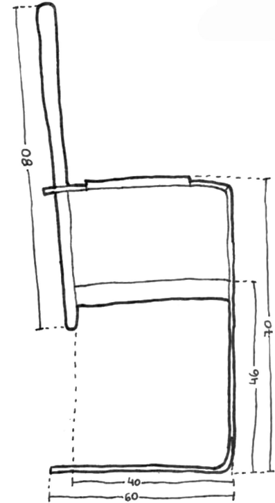
ELEVATION SCALE 1:10
