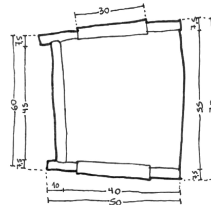
PLAN SCALE 1:10
